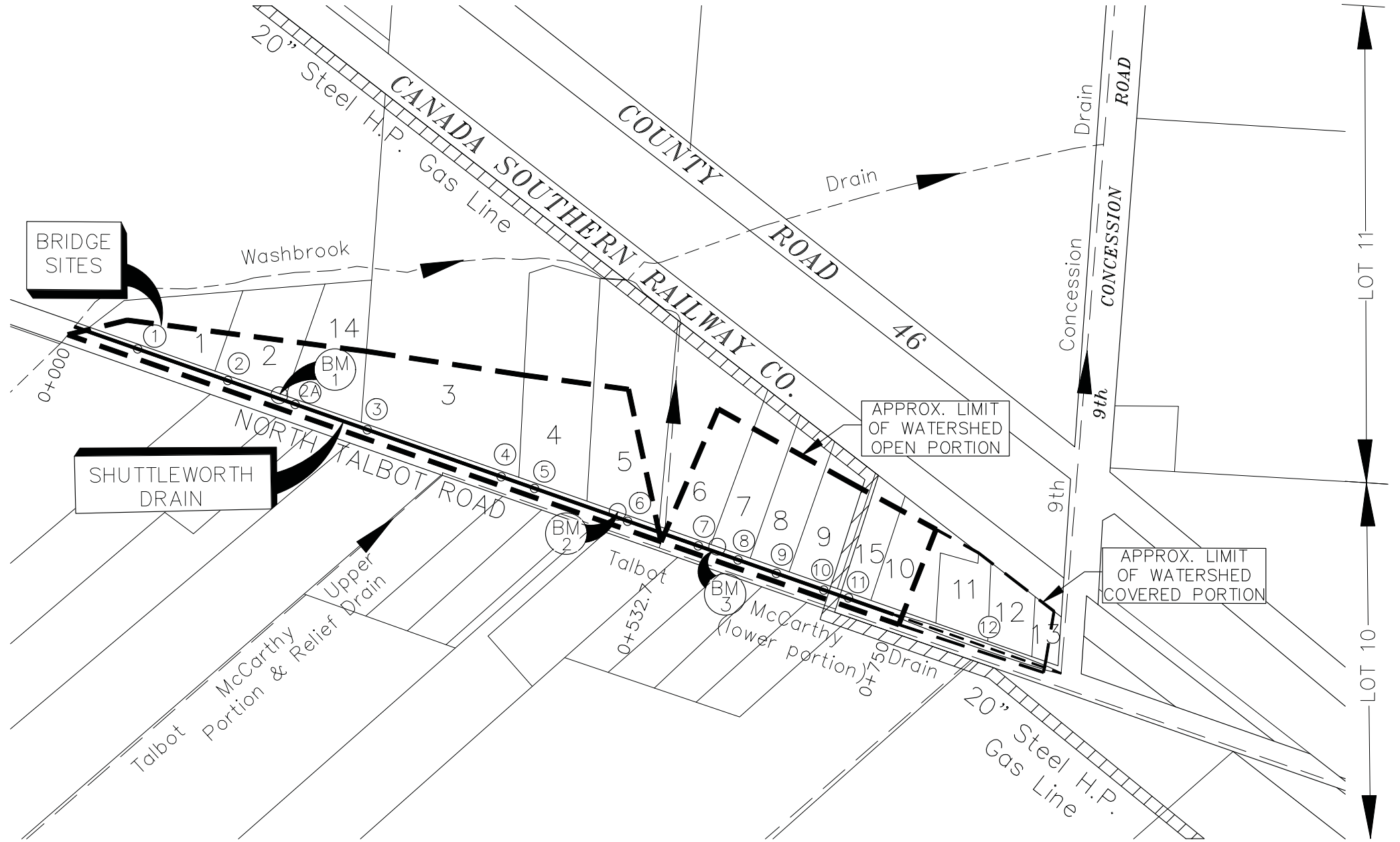
SHUTTLEWORTH DRAIN WATERSHED PLAN Scale = 1:2,000
