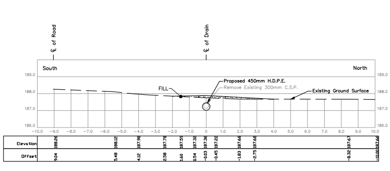
STA. 0+262.8 Scale = 1:100
